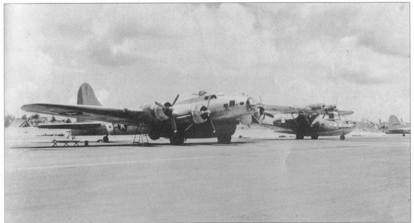
ABOVE: an unnamed B-17 of the 4th Emergency Rescue Sq., Seventh Ftr. Comd., on Iwo Jima late in the Pacific war. The dark shape under the fuselage is a motor launch, and a radar unit replaces the chin turret. BELOW: NINE O NINE was a 71 mission veteran with the 323rd Sq., 91st Bomb Grp., Eighth Air Force.
